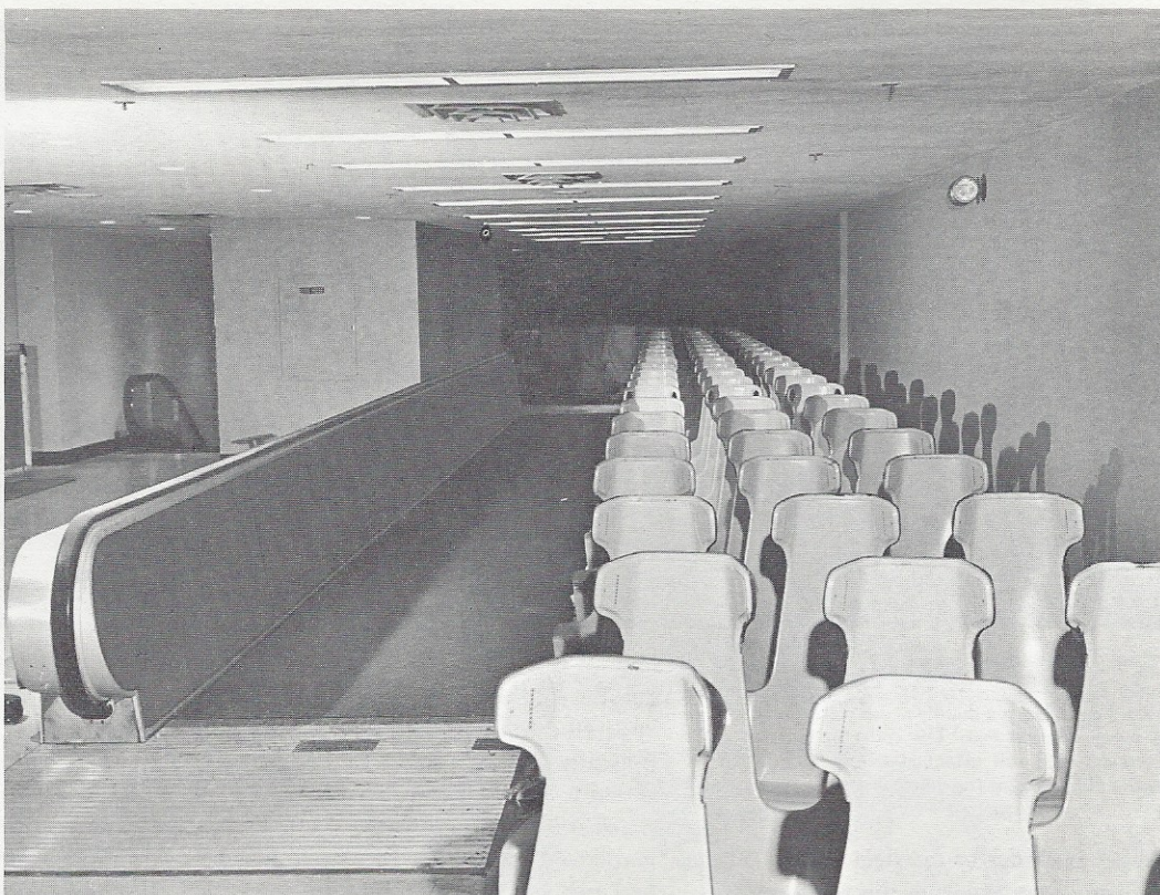
Fig. 10 — Loading and unloading of passengers is accomplished by two moving belt walkways running parallel to the track and moving at the same speed as the ride. One of the walkways is shown here.
