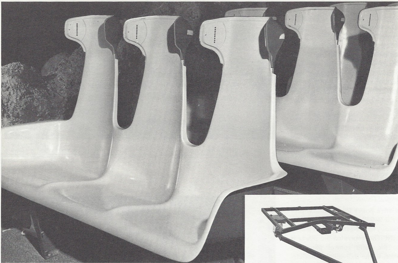
Fig. 7—Each of the 463 seats accommodates three passengers. Each passenger headrest contains two speakers connected to a sound reproducing unit (Fig. 9) located beneath every third seat. The seat is set on a carpeted platform and is attached to a steel chassis (inset).
