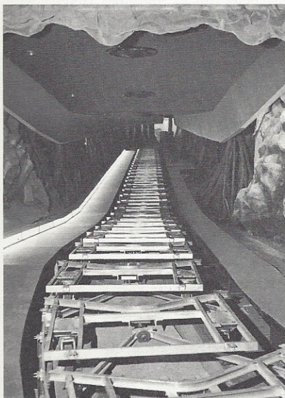
Fig. 3—A service walkway parallels the entire length of the track. This walkway is automatically lighted in case of emergency, as shown in this photograph taken during construction. Cardboard dust shields, used temporarily during the construction period, appear over the continuous center opening of the track.
